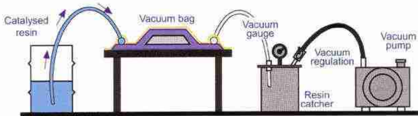
INFUSION SET UP SCHEMATIC
